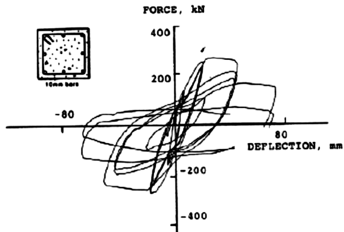
a) Poorly confined column
